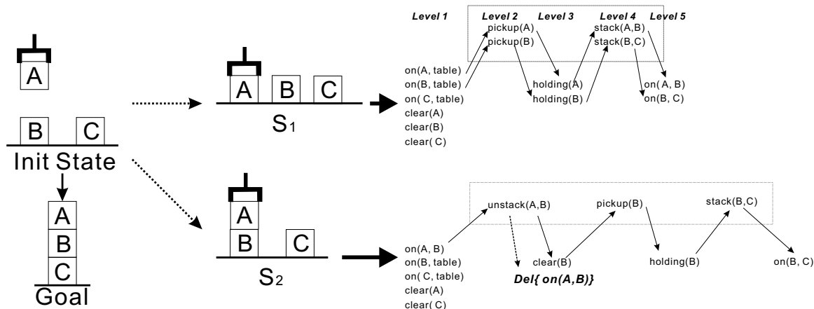
Figure 1: Blockworld Example
