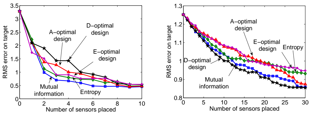
(a) Comparison with A-, D- and E-optimality on temper- (b) Comparison with A-, D- and E-optimality on precip- ature data itation data, 111 node subsample
