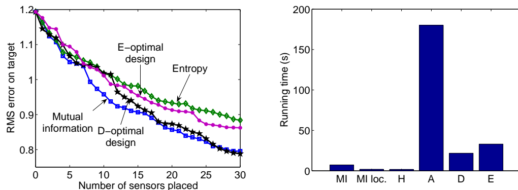
(c) Comparison with D- and E-optimality on precipita- (d) Running time for 111 node precipitation subsample tion data
