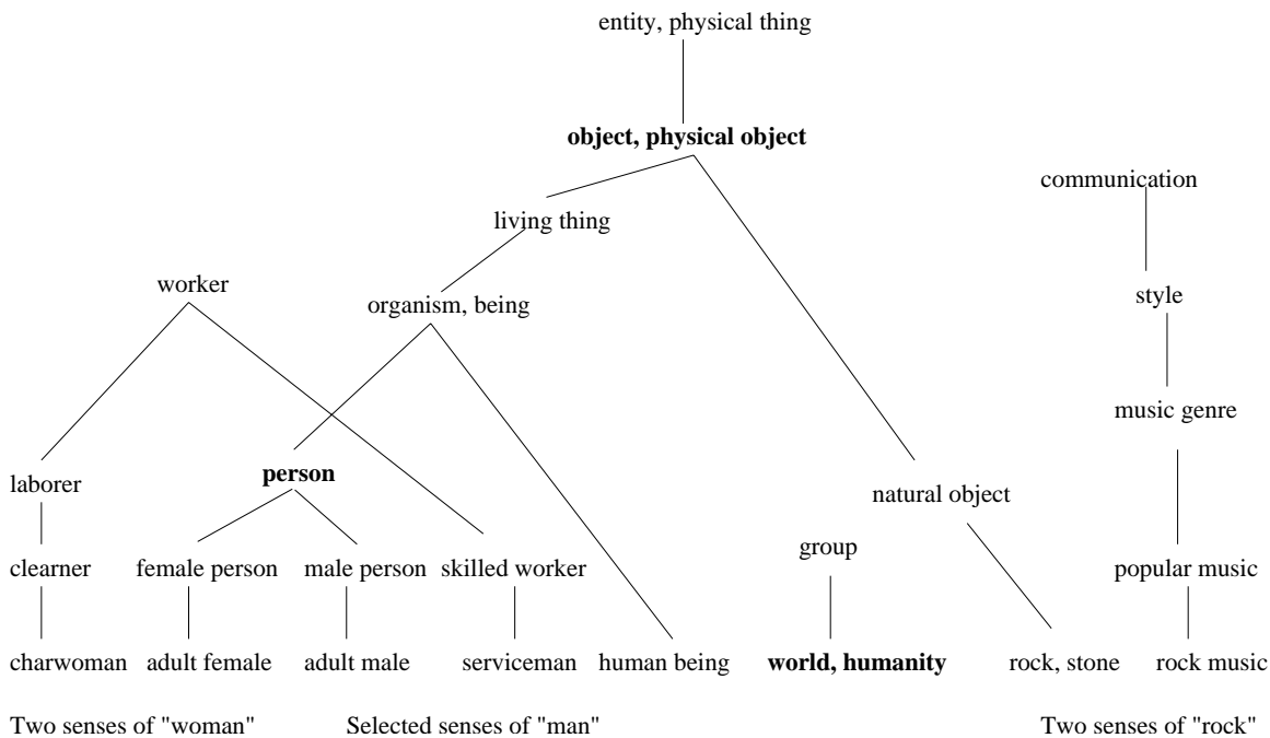
Figure 6: Portion of the WordNet hypnym hierarchy showing three different generalizations of the word “man”
