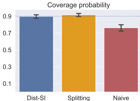
Figure 1: Coverage probabilities of “Dist-SI” (our procedure for selective inference with distributed data), the “Splitting”, and “Naïve” methods for a Gaussian linear model, with 2 local machines and a central machine. The 2 local machines and the central machine each have 1000 samples. The pre-specified level of coverage is 0.90, as indicated by the dotted horizontal line at 0.9.
