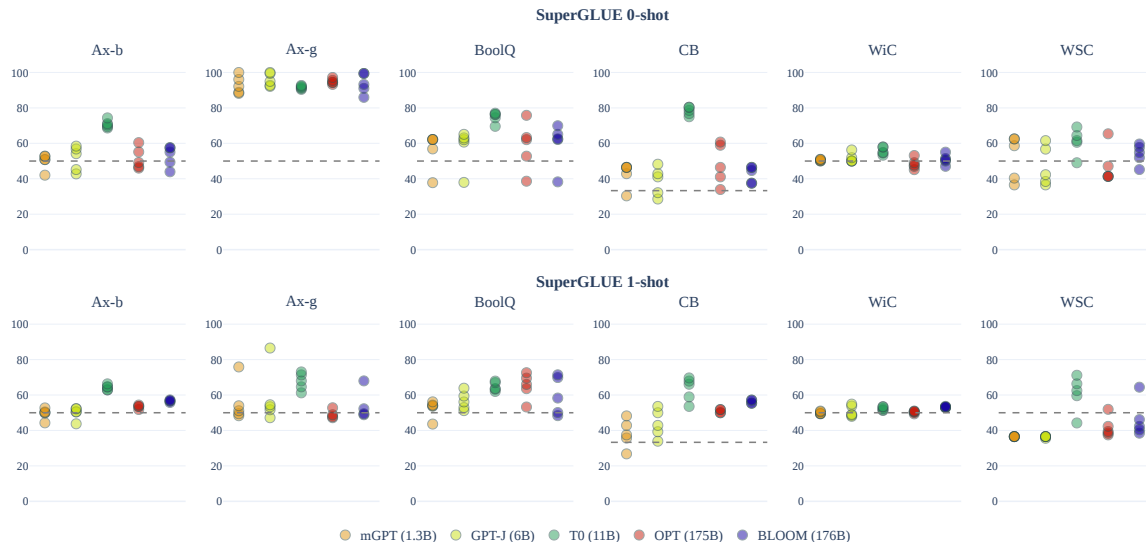
Figure 7: Performance of various LLMs on subset of tasks from SuperGLUE benchmark in zero- and one-shot prompt-based setting. Each point represents a different prompt for a given dataset.
