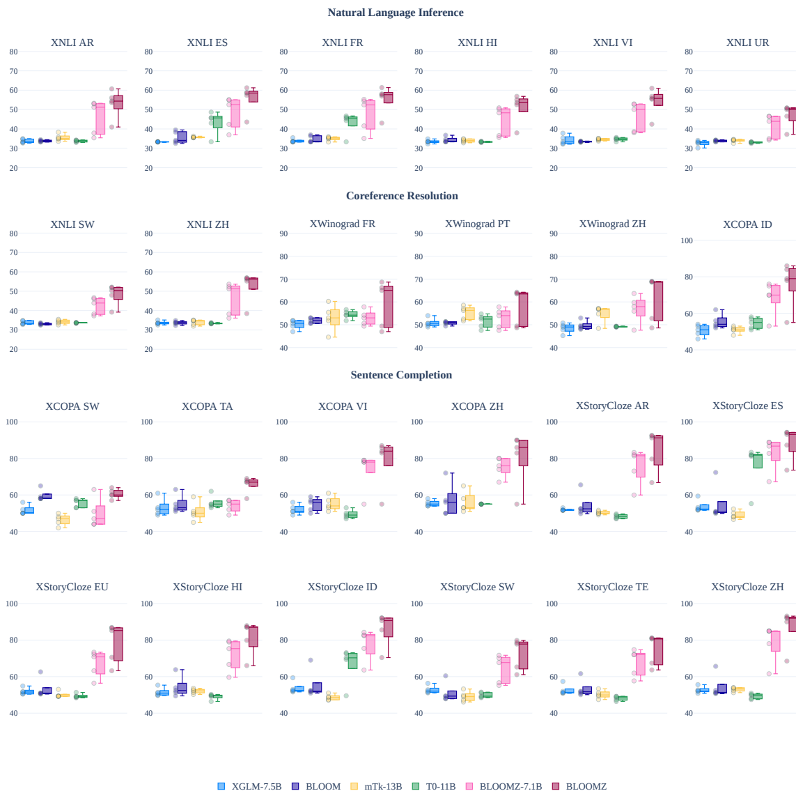
Figure 11: BLOOMZ zero-shot task generalization. Five untuned prompts are evaluated for each dataset and plotted. T0-11B is monolingual (English) while other models are multilingual. T0 performance may be hurt by its inability to tokenize some non-English texts.
