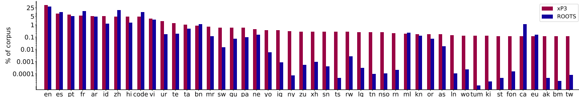
Figure 4: Language distribution of the prompted dataset xP3 closely follows ROOTS.
