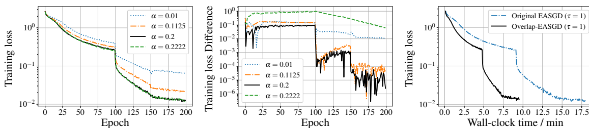
(a) Average training loss of local models. (b) The difference of training loss between workers and the auxiliary variable. (c) Benefit of using auxiliary variable: overlapping communication and computation.
