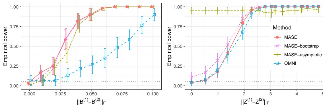
Figure 8: Empirical power for rejecting the null hypothesis that two graphs have the same distribution as a function of the difference in their parameters at a 0.05 significance level (black dotted line). Both graphs are sample from a mixed-membership SBM \mathbf{A}^{(i)} \sim \text{MMSBM}(\mathbf{Z}^{(i)}, \mathbf{B}^{(i)}) . In the left panel, the community assignments \mathbf{Z}^{(1)} and \mathbf{Z}^{(2)} are the same, while the connection probability changes on the x-axis. In the right panel, \mathbf{B}^{(1)} = \mathbf{B}^{(2)} , while the community assignments of a few nodes change. Both methods improve their power as the difference between the graphs get larger, but MASE can effectively use the common subspace structure to outperform OMNI when the difference between the \mathbf{B} matrices is small. The p-values of MASE are estimated accurately using a parametric bootstrap, while the asymptotic distribution is only valid in the first scenario when the common invariant subspace is represented in both graphs.
