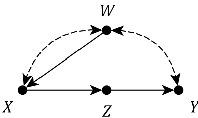
Figure 2: A graph G for the example on the use of simplification sets.
